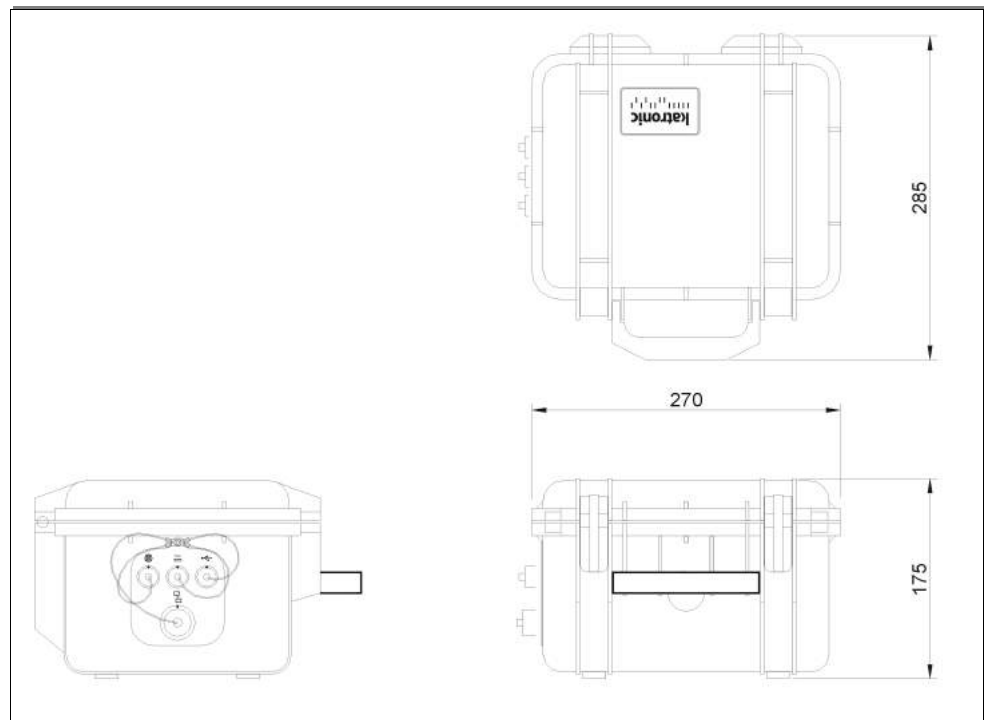
Drawing 1: Outline dimensions
