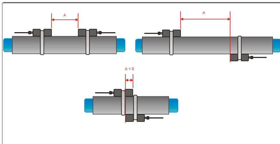
Illustration 6: Sensor pipe mounting configurations
