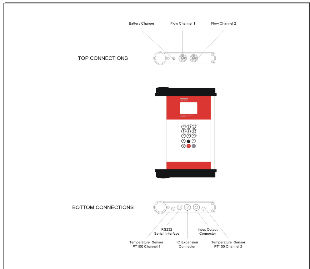
Drawing 3: Electrical connections overview KATflow 230
