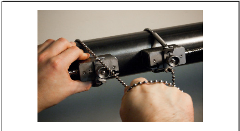
Illustration 8: Correct positioning of the sensors
