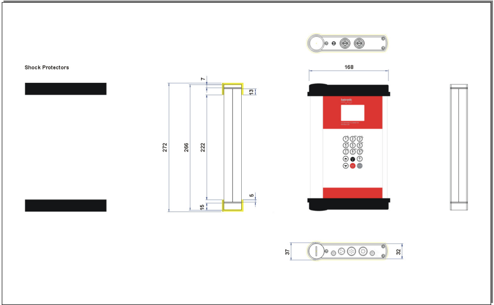
Drawing 1: Outline dimensions KATflow 230
